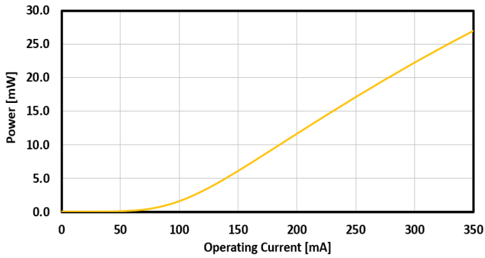
FIG. 5: SLED 2 OUTPUT POWER VS CURRENT
